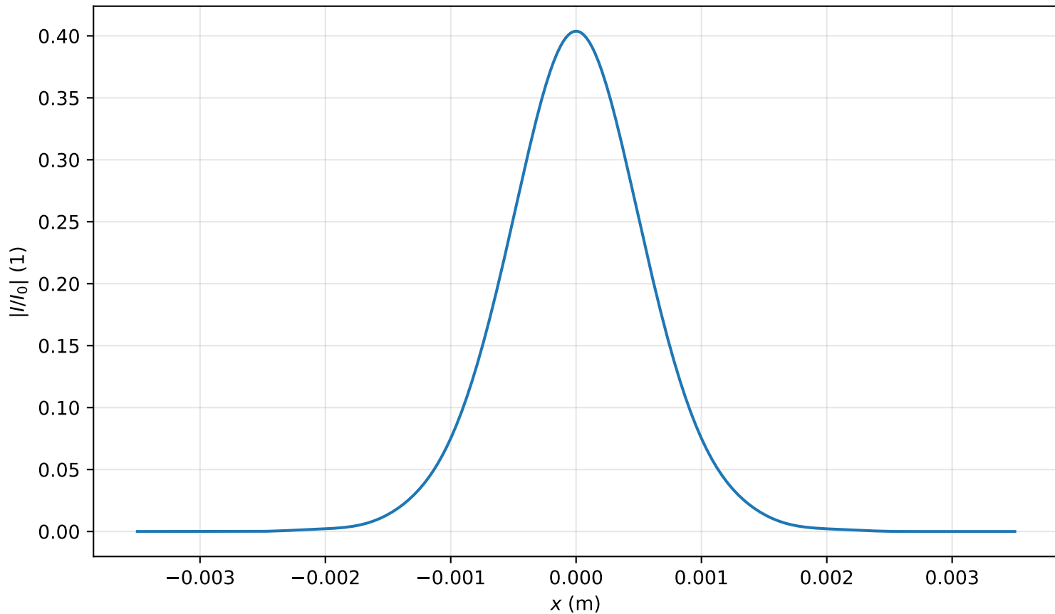
Intensity profile I(x, y = 0, z = 3.901m)/I_0 , P_{in}=0.5P_{cr} , artificial time
